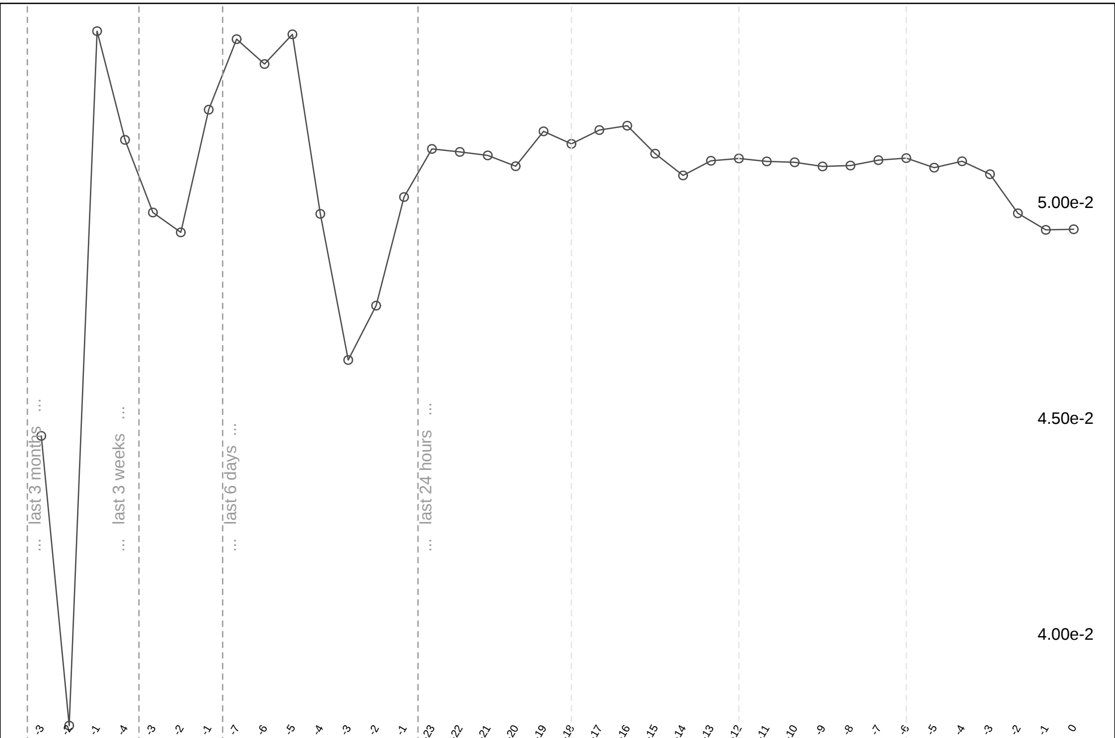
CryptoMarketPlot.com: log timeline of Maker on 4 months, updated at 2020/07/31 17:48 UTC
